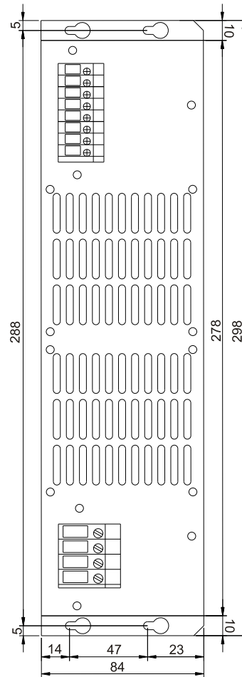
Vista Frontal
